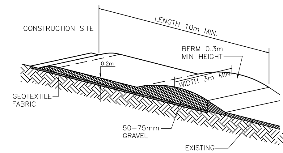
DETAIL 2 TEMPORARY CONSTRUCTION EXIT
