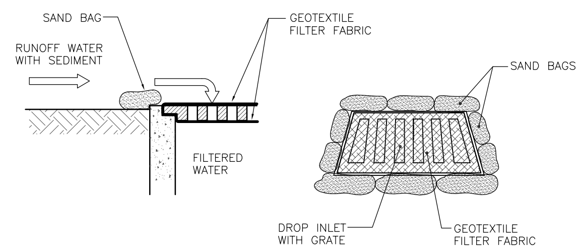
DETAIL 3 GEOTEXTILE FILTER FABRIC DROP INLET SEDIMENT TRAP
