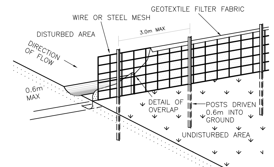
DETAIL 1 SEDIMENT FENCE
